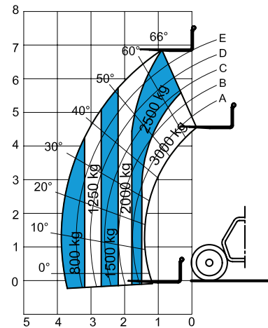
Lift capacity chart with floating forks****
