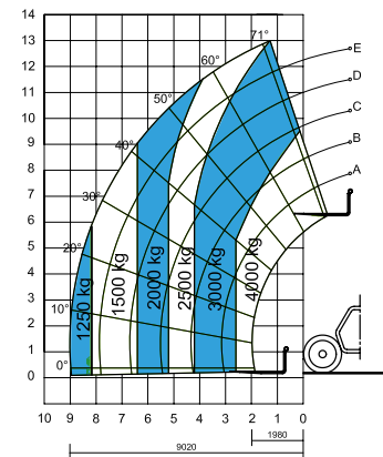
Lift capacity chart (with outriggers)****
