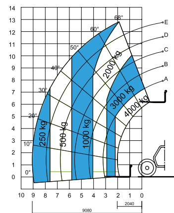
Lift capacity chart (without outriggers)****
