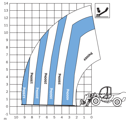
Lift capacity chart (with stabilisers)
